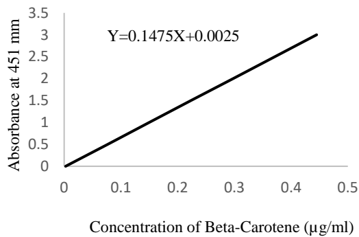
Figure 2: Standard curve of beta carotene (carrot) graph for determination of sample concentration (Javer et al., 2013)
