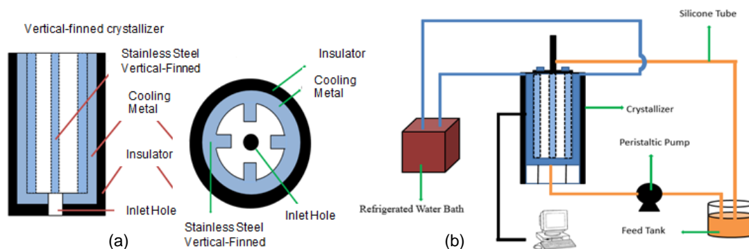
Figure 1: (a) Inner structure and upper view of VFC (b) Experimental set-up
