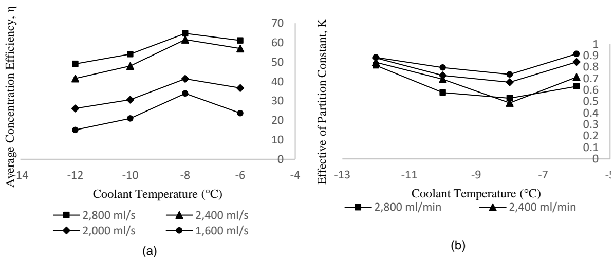
Figure 3: (a) Average Concentration Efficiency, \eta vs Coolant Temperature ( ^{\circ}\text{C} ) and Circulation Flowrate (b) Effective Partition Constant, K vs Coolant Temperature ( ^{\circ}\text{C} ) and Circulation Flowrate.
