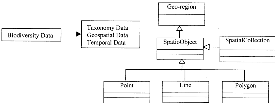
Figure 4: Object type and spatial data as object
