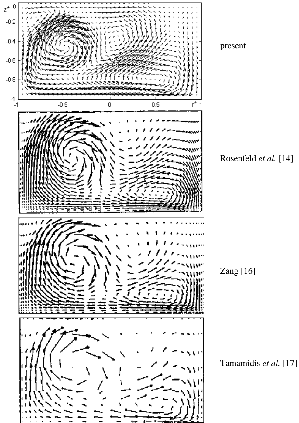
Figure 4g: Secondary velocity vectors plot for De=520 along a duct of H_D/R_o=0.4348 and \gamma=1 at \theta=90^\circ
