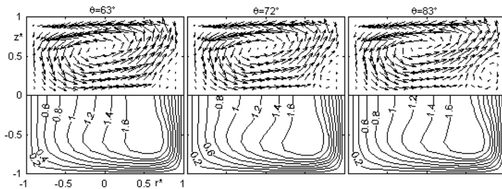
Figure 3b: Contour plots of U_\theta/U_0 and secondary velocity vectors plots for De=142 along a duct of H_D/R_0=0.0274 and \gamma=1 at \theta=63^\circ , \theta=72^\circ and \theta=83^\circ
