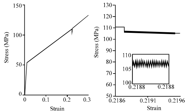
Fig. 3: FE model showing an interval of RU excitation for a constant coefficient of friction \mu = 0.25 , inset shows zoomed view of oscillatory stress amplitude
