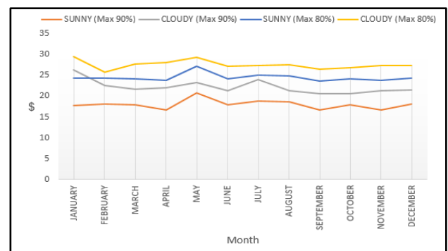
Figure 11 Battery SoC and MT cost for 1 year
