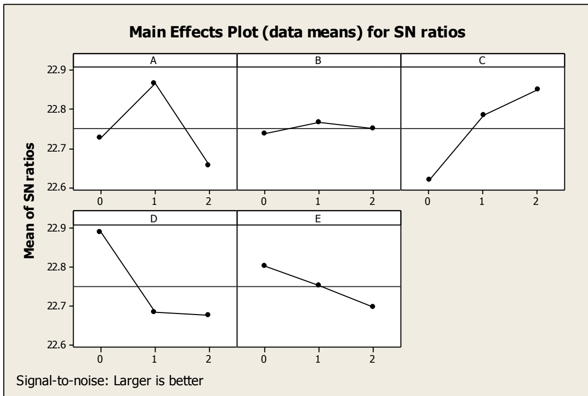
Figure 2 : Main effects plot(data means) for S/N ratio
