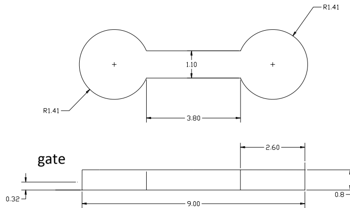
Figure 1 : Micro mold dimension in mm
