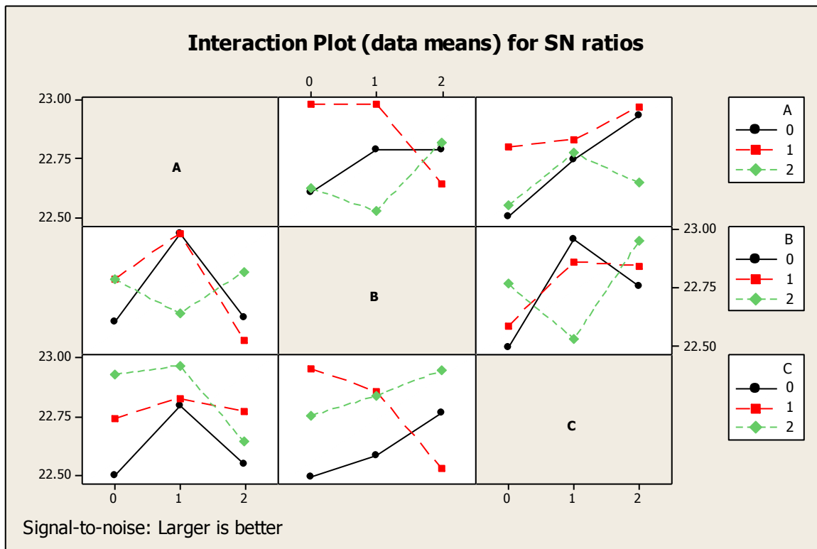
Figure 3 : Interaction plot(data means) for S/N ratio
