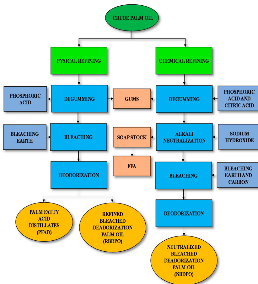
Figure 3. Chemical and physical refining process of palm oil.
