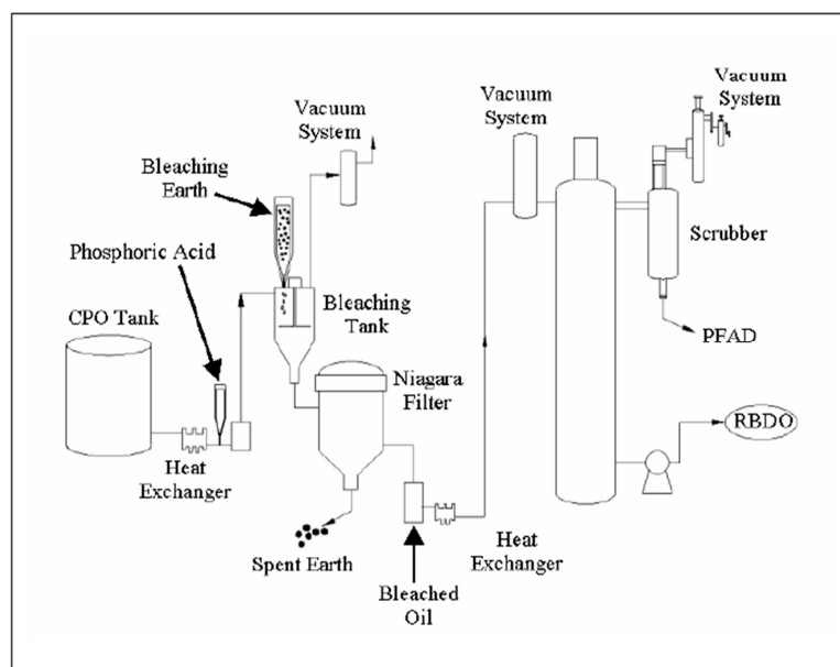
Figure 4. Physical refining process [2].
