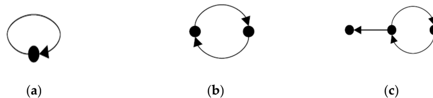
Figure 7. (a) A 1-cycle and ACS; (b) A 2-cycle and ACS; (c) An ACS but not irreducible.
