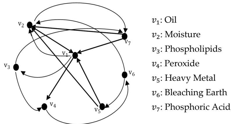
Figure 8. Graph G_p .
