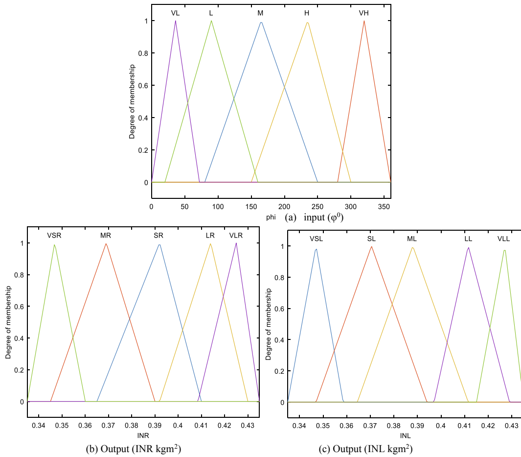
Fig. 11. Membership functions for inertia estimation using fuzzy logic.
