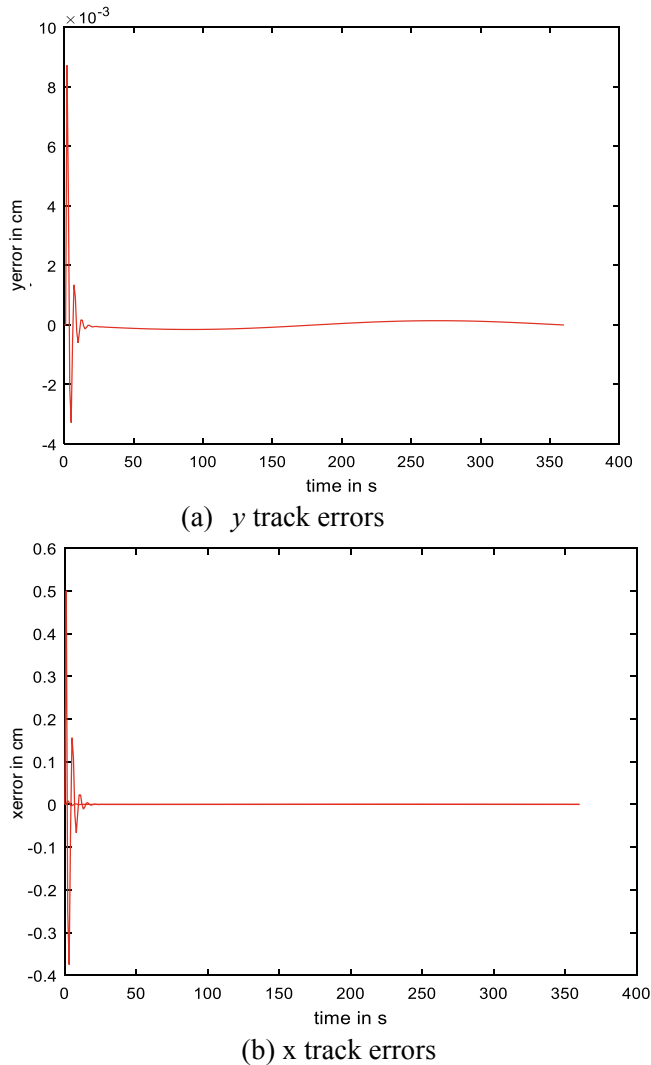
Fig. 22. Real-time WMR tracking errors when moving in a circular path.
