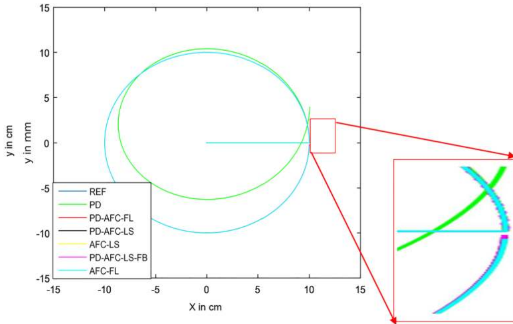
(a) the trajectory of all controllers
