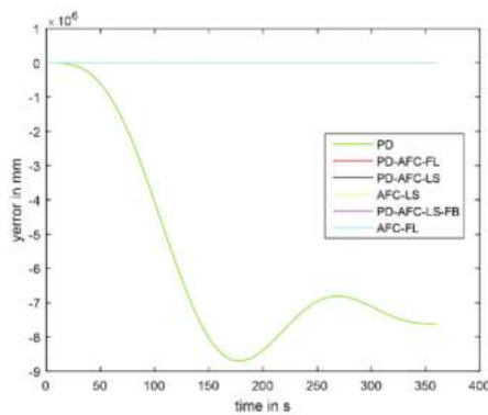
(b) y track errors for all controllers
