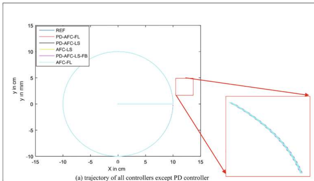
Fig. 17. Results of all controllers' schemes in a circular path with disturbance.
