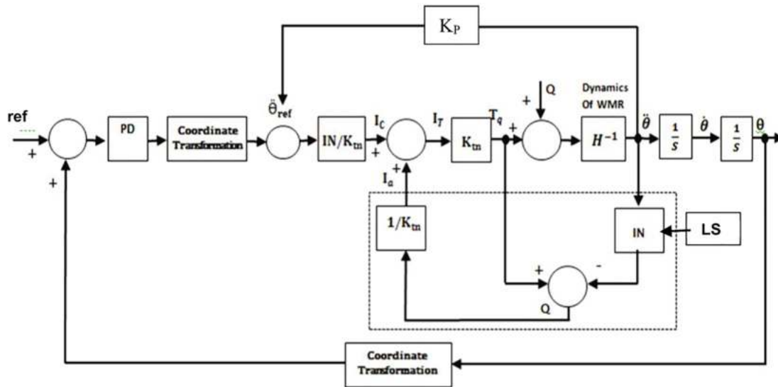
Fig. 10. PD-AFC Controller with Laser Simulator Logic and Quick Feedback compensation loop.
