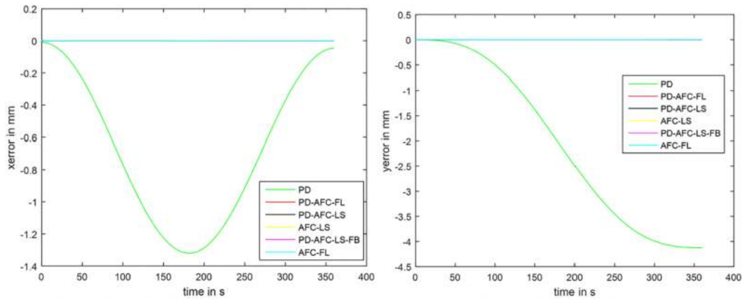
(b) y track errors for all controllers
