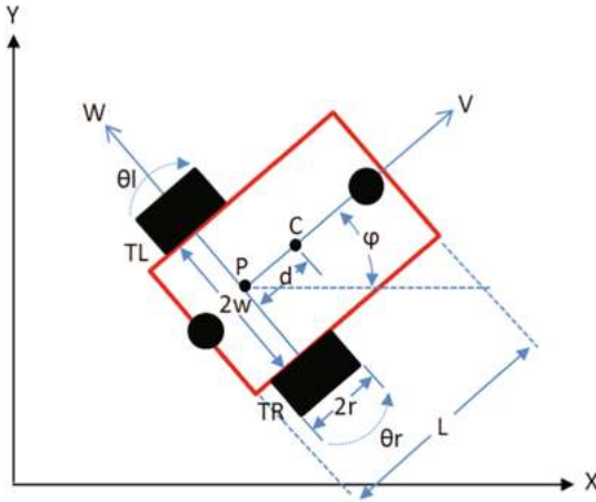
Fig. 9. Local /global coordinate system with wheeled mobile robot.
