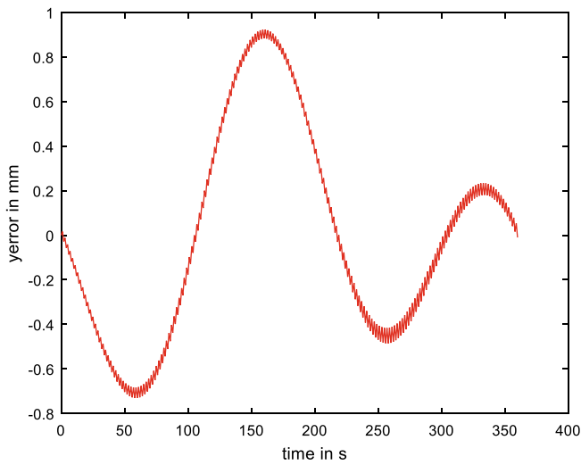
(a) y track errors
