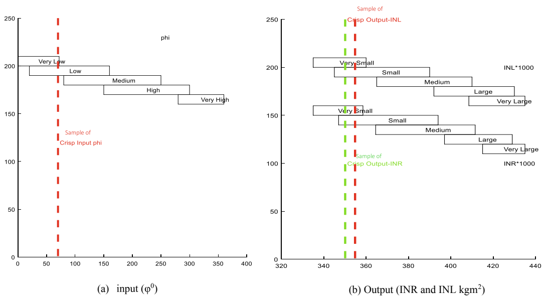
Fig. 12. Membership functions for inertia estimation using laser simulator logic.
