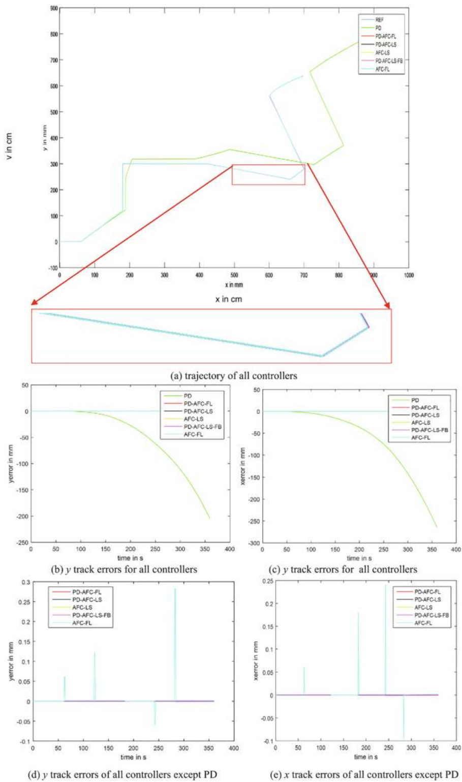
Fig. 14. Results for all controller schemes in zigzag path without disturbance.
