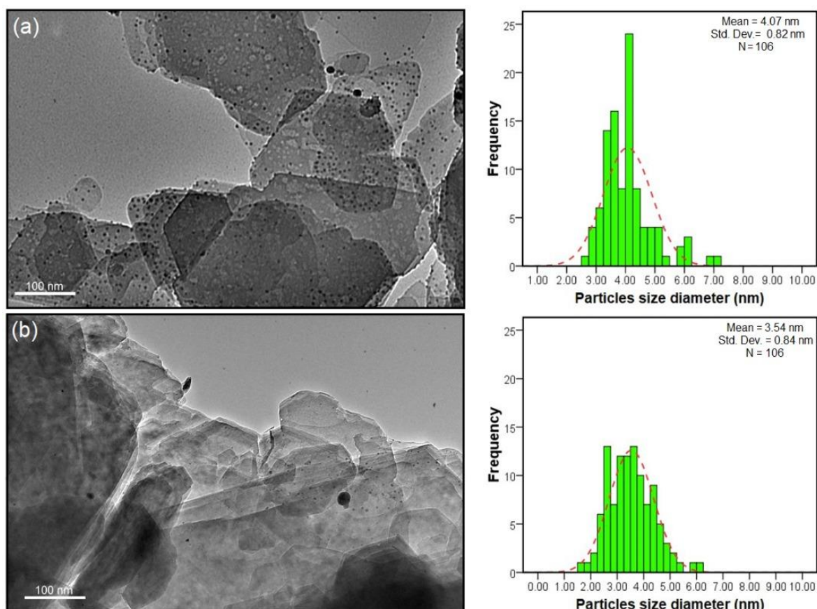
Fig. 2. TEM image of spherical Ag/KIn NCs prepared by (a) \gamma -irradiation and (b) \text{NaBH}_4 methods.
