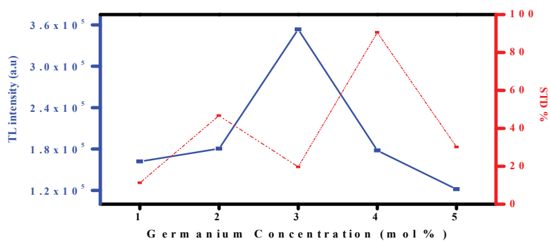
Fig2. TL intensity and standard error of Al 2 O 3 : Ge with different concentration
