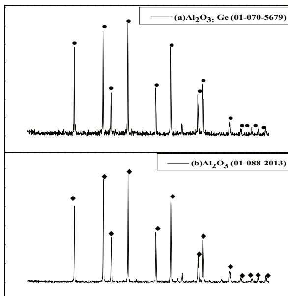
Fig1. XRD pattern of (a) Al 2 O 3 doped 3 mol % Ge samples and (b) un-doped Al 2 O 3
