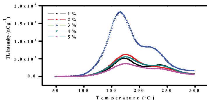
Fig3. TL glow curve of \text{Al}_2\text{O}_3 : Ge at different mole concentration exposed to 50 Gy Cobalt-60
