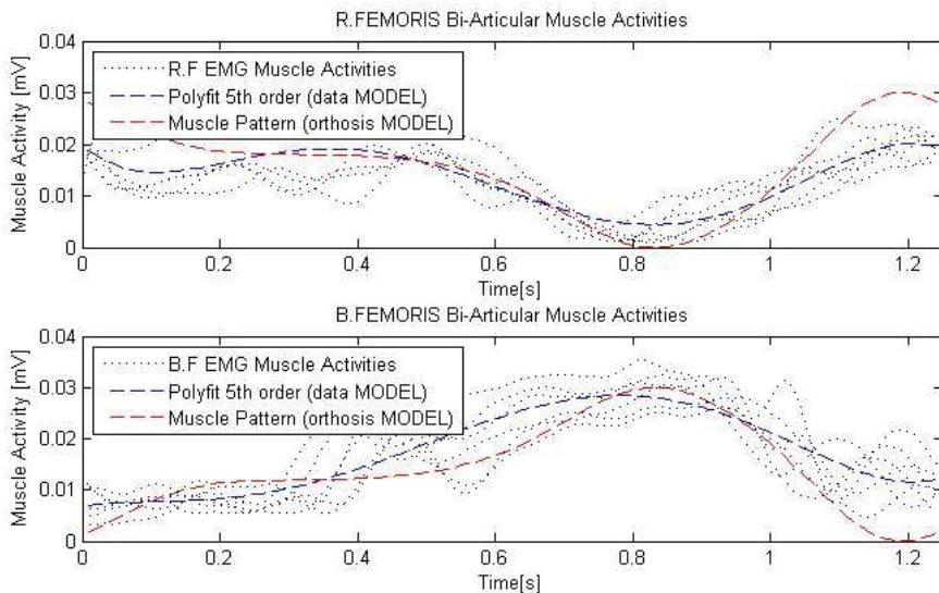
Fig. 3. Evaluation of the bi-articular muscle’s mathematical model with the Rectus Femoris (RF) and Bicep Femoris (BF) muscle activities.
