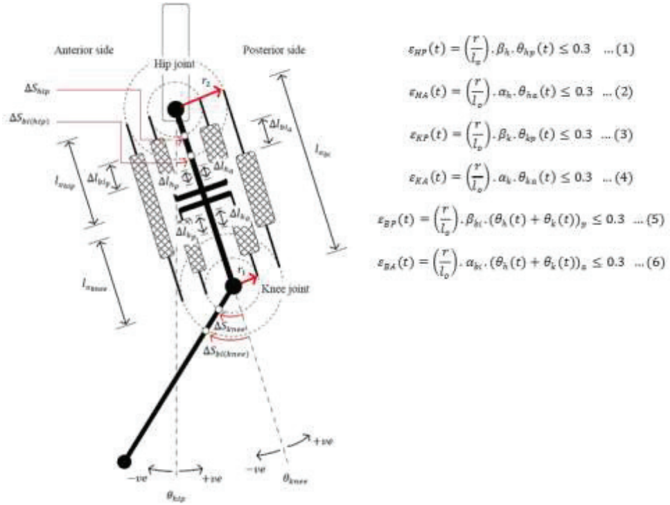
Fig. 1. Pneumatic muscle actuated lower limb orthosis simplified model for mono- and bi-articular muscles between hip and knee joints; where, \varepsilon_{HA} and \varepsilon_{HP} are the anterior-posterior muscle contraction of the hip joint; \varepsilon_{KA} and \varepsilon_{KP} are the anterior-posterior muscle contraction of the knee joint; \varepsilon_{BA} and \varepsilon_{BP} are the anterior-posterior muscle contraction of the bi-articular muscle (hip and knee joint); \alpha and \beta are muscle activation level for the anterior-posterior muscles; \theta_H and \theta_K are hip and knee joints.
