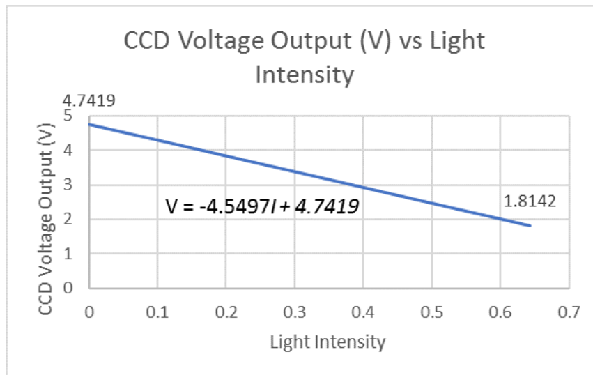
Figure. 2. Graph CCD voltage output versus light intensity
