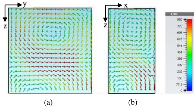
FIGURE 9. E-field distribution of the proposed configuration (a) TE_{10}^x at 3.82 GHz and (b) TE_{10}^y at 4.4 GHz.
