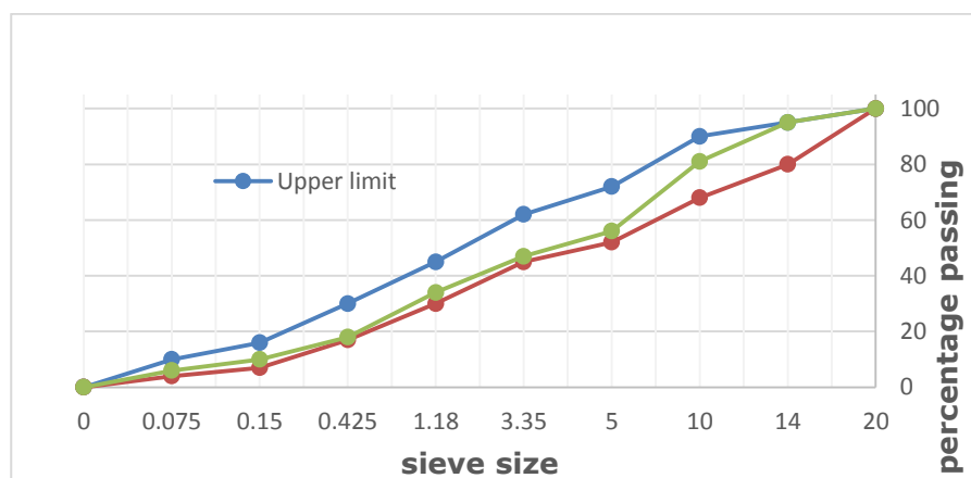
Fig 1. Sieve Analysis
