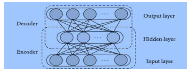
FIGURE 6. Stacked auto-encoders.
