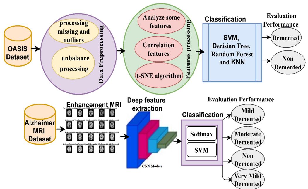
Figure 1. Methodology for classifying the OASIS and MRI Alzheimer's datasets.
