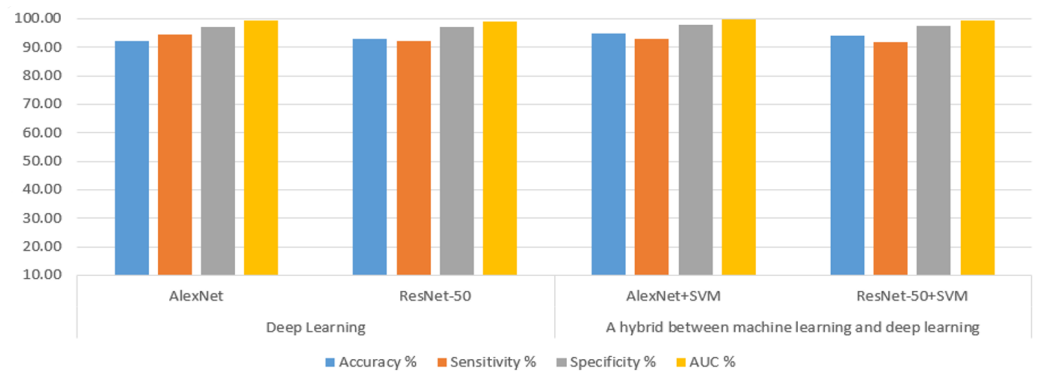
Figure 8. The performances of deep learning and hybrid techniques.
