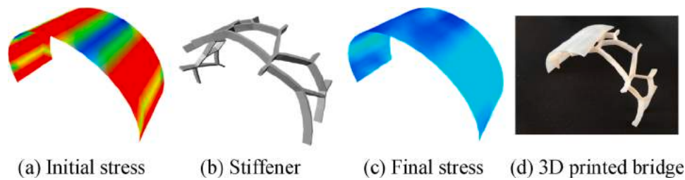
Fig. 17. Unstiffened and stiffened Bridge.
