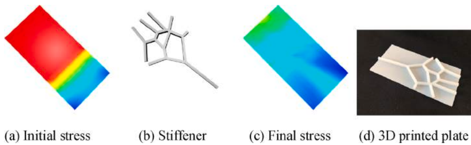
Fig. 13. Unstiffened and stiffened Plate.
