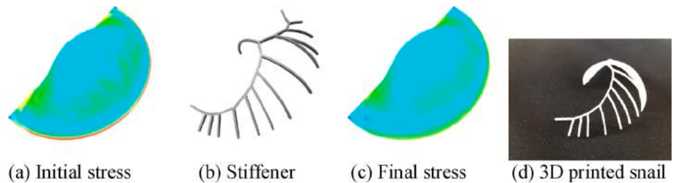
Fig. 15. Unstiffened and stiffened Snail.
