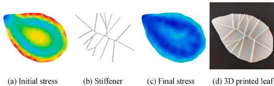
Fig. 21. Unstiffened and stiffened Leaf.
