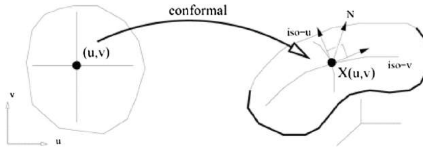
Fig. 3. Conformal mapping from a 2D point (u, v) to a surface point X(u, v) [40].
