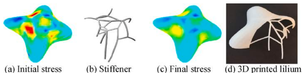
Fig. 20. Unstiffened and stiffened Lilium.
