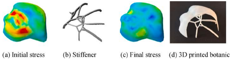
Fig. 14. Unstiffened and stiffened Botanic.
