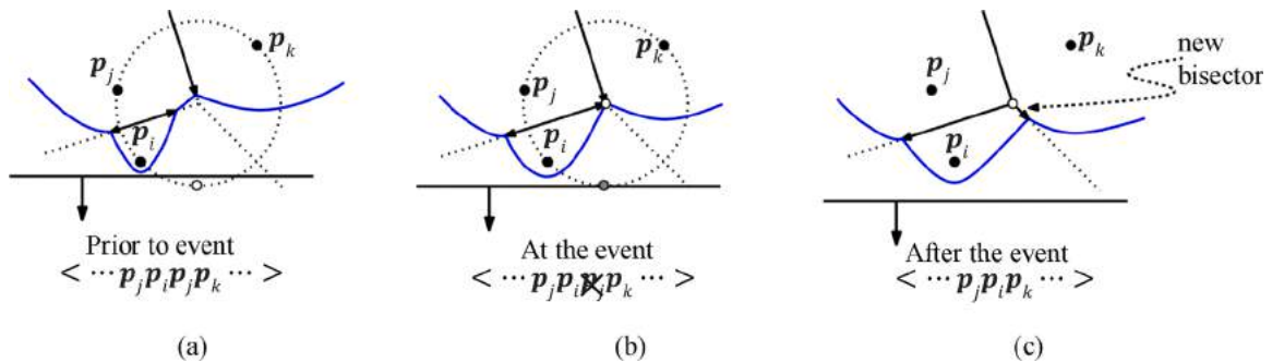
Fig. 7. Circle event.
