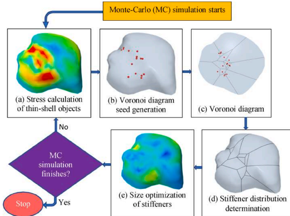
Fig. 1. Algorithm overview.
