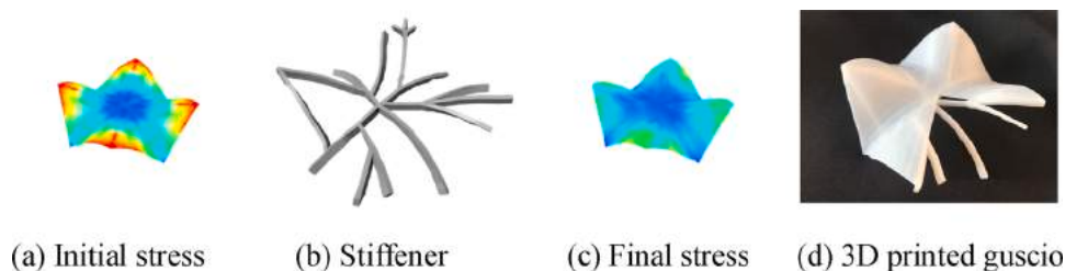
Fig. 19. Unstiffened and stiffened Guscio.
