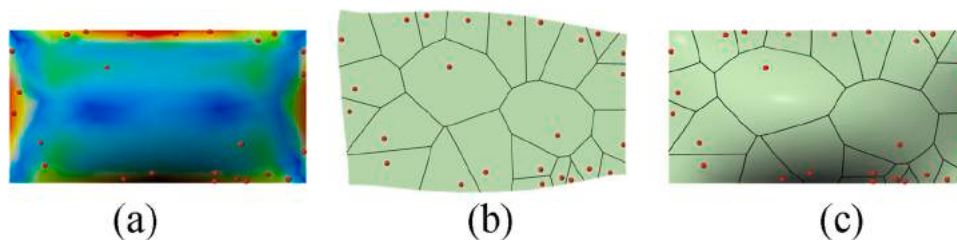
Fig. 8. Generation of Voronoi diagram.
