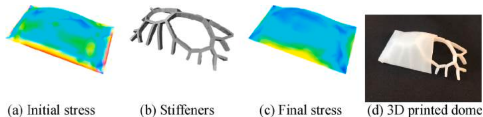
Fig. 16. Unstiffened and stiffened Dome.
