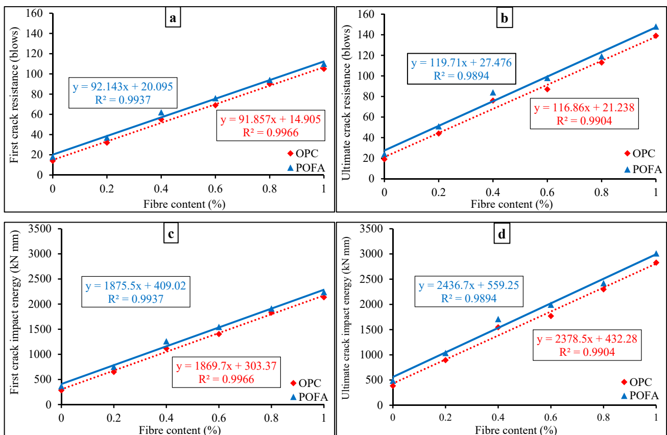
Figure 17. Correlations between (a) first crack resistance, (b) ultimate crack resistance, (c) first crack impact energy, and (d) ultimate crack impact energy vs fibre content of concrete containing WPFT fibres at first and ultimate cracks.
