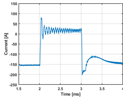
(a) power winding d Current—proposed.
