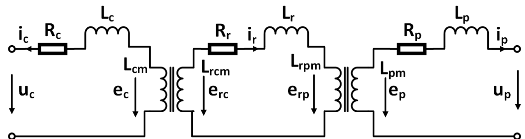
Figure 2. Brushless doubly-fed induction generator equivalent circuit.
