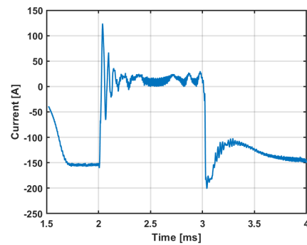
(c) power winding d Current—Zhang et al.
