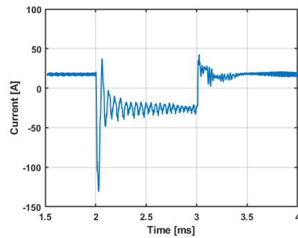
(a) power winding q Current—proposed.
