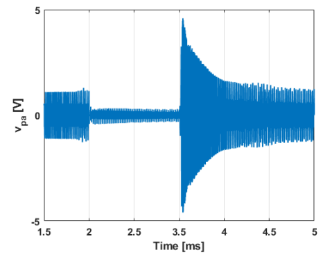
(b) power winding Voltage—Tohidi et al.
