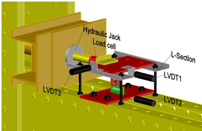
Figure 3 3D view of the test set up.
