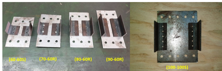
Figure 1 Test specimens.
