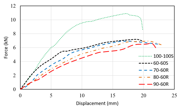
Figure 6 Force-displacement relationships.
