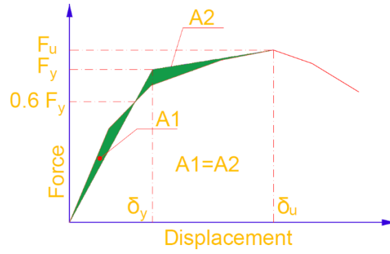
Figure 7 Bilinear representation of force-displacement relationships.
