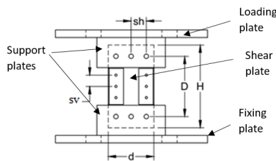
Figure 2 Details of constructed shear plates.
