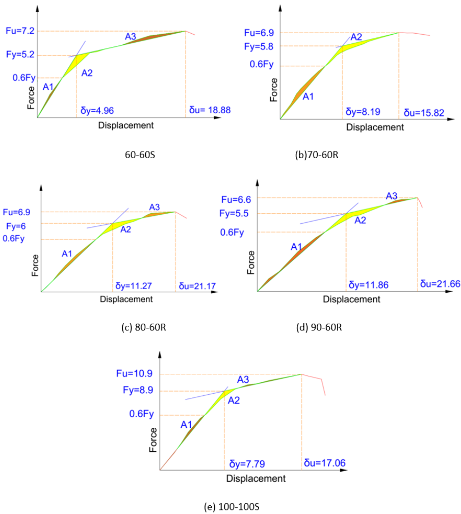
Figure 8 Bilinear representation of backbone curves.
