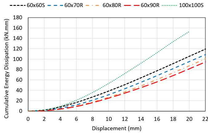
Figure 9 Energy dissipation of tested dampers.
