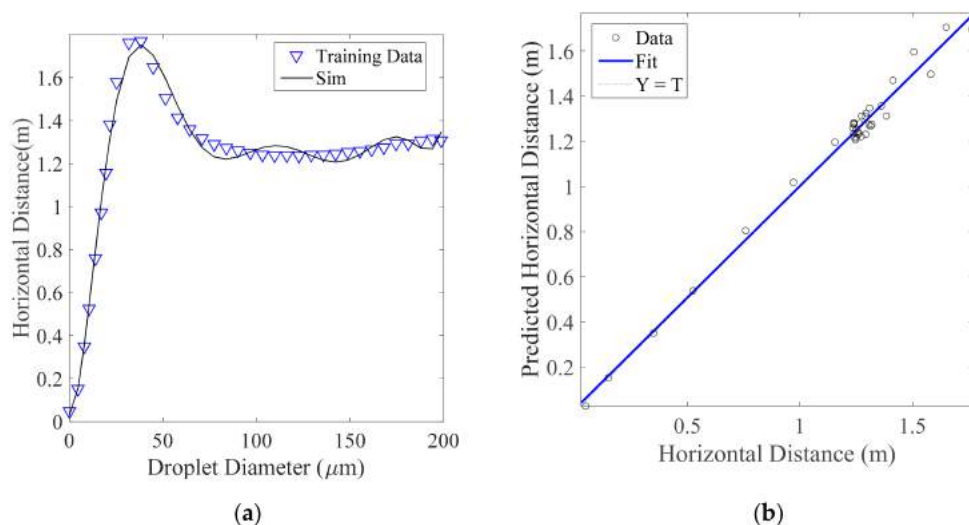
Figure 11. The horizontal distance prediction compared to the numerical model as a function of droplet diameter (a) and the training correlation (b).
