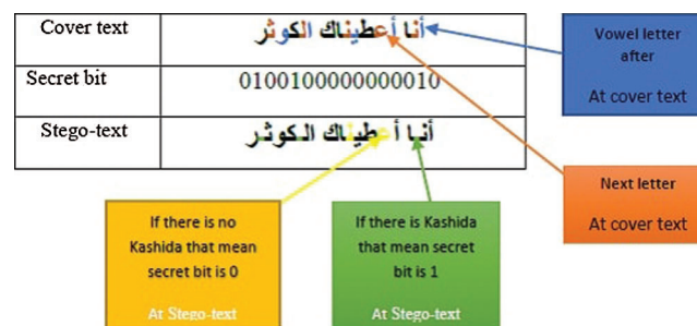
Figure 15: Extracting the secret bits
