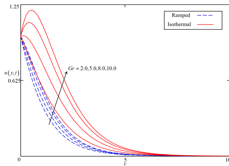
Figure 16. Consequence of Gr on u(y, t) when \alpha = 0.5 , \phi = 0.04 , \beta = 0.5 , M = 0.5 , Nr = 0.5 , and \omega t = 0.15 for spherical case.
