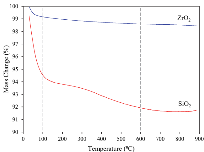
Figure 6. TGA curve for SiO_2 and ZrO_2 nanopowder.
