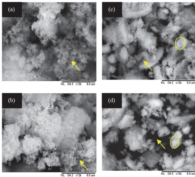
Figure 7. SEM micrographs of (a) uncalcined \text{SiO}_2 nanopowder, (b) \text{SiO}_2 nanopowder calcined at 900\text{ }^\circ\text{C} , (c) uncalcined \text{ZrO}_2 nanopowder, (d) \text{ZrO}_2 nanopowder calcined at 900\text{ }^\circ\text{C} . The arrow indicates loosely bound agglomeration while the circle indicates closely bound aggregation.
