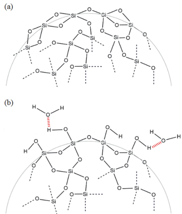
Figure 3. Surface of SiO 2 with (a) Q 4 conformations, (b) Q 3 conformations.
