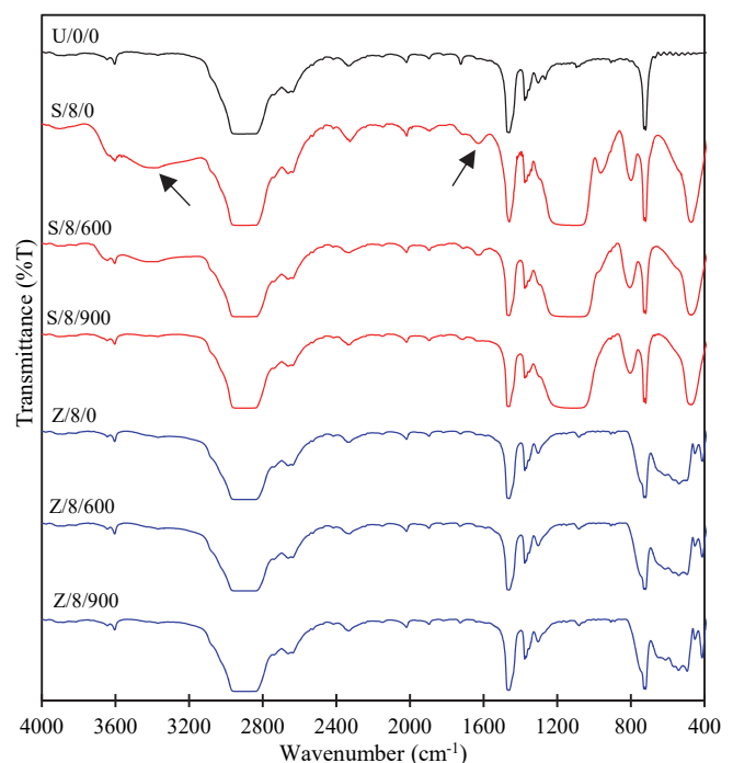
Figure 8. FTIR spectra comparing unfilled PE and nanocomposites containing uncalcined and calcined \text{SiO}_2 and \text{ZrO}_2 .
