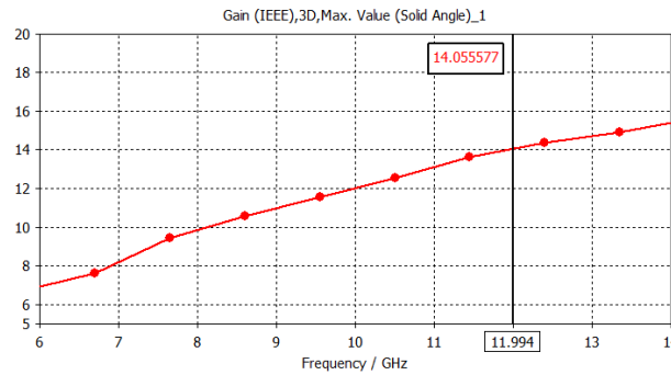
Figure 11. Gain versus frequency plot for Horn antenna design
