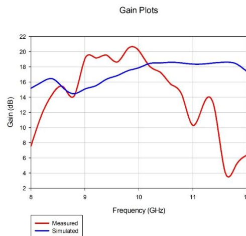
Figure 13. Simulated and measured gain versus frequency plot for proposed transmitarray antenna
