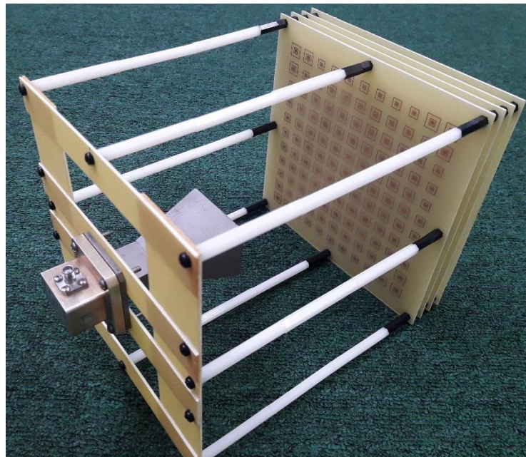
Figure 5. Prototype of FSS Transmitarray antenna
