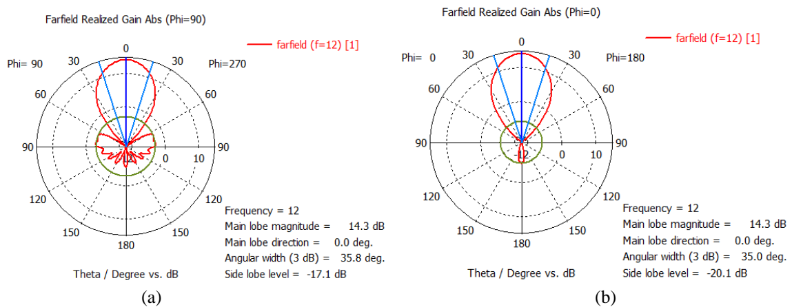
Figure 10. The radiation pattern for Horn antenna at 12GHz (a) E-plane (b) H-plane
