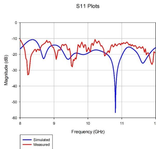
Figure 12. Simulated and measured S11 magnitude (dB) plots for proposed transmitarray antenna
