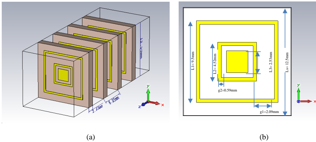
Figure 2. Isotropic and top views of Multi-layer FSS unit cell
