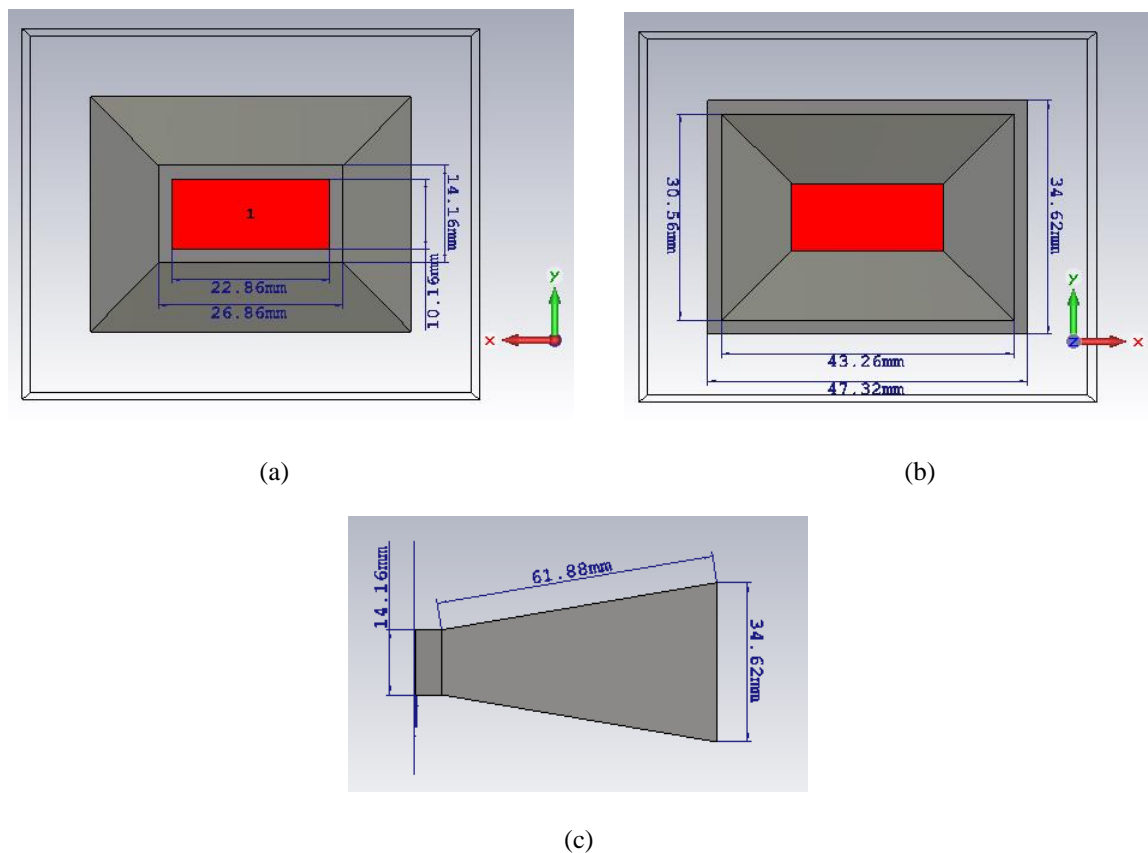
Figure 3. X-band horn antenna with rectangular waveguide section (a) Bottom (b) Top (c) Side view
