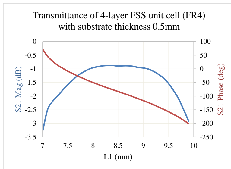
Figure 7. S_{21} magnitude and phase plots for unit cell design on substrate thickness = 0.5mm
