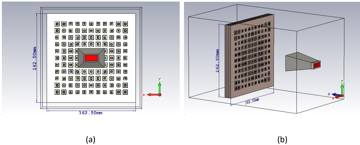
Figure 4. M-FSS type transmitarray antenna design (a) Top (b) Isotropic views
