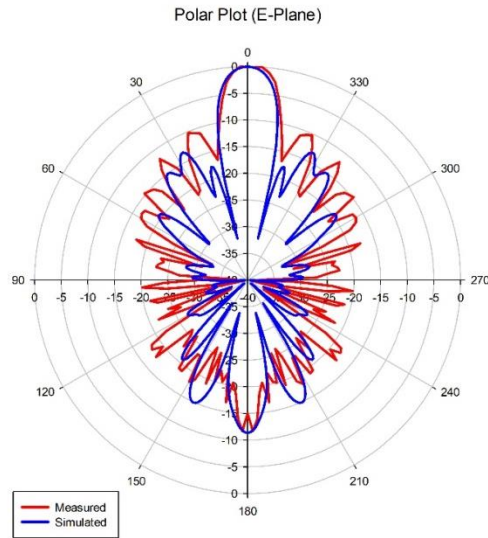
Figure 14. Comparison of simulated and measured radiation pattern (Polar Plot) for the double square ring with center patch transmitarray antenna at peak gain
