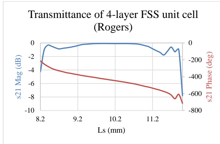
Figure 8. S21 magnitude and phase plots for unit cell design using Rogers RT/Duroid 5880 substrate with thickness 1.6mm
