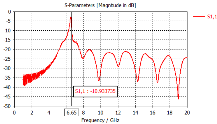
Figure 9. S11 magnitude (dB) plot for Horn antenna design
