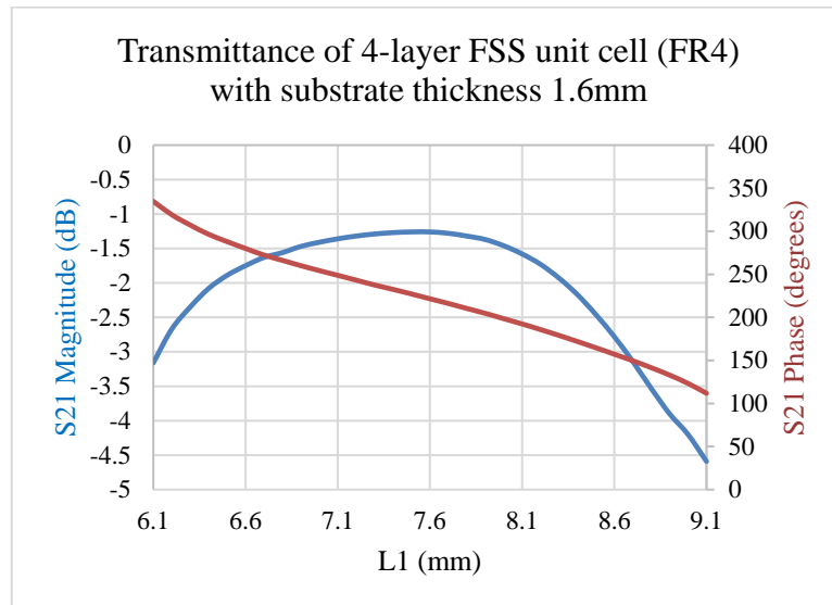
Figure 6. S_{21} magnitude and phase plots for unit cell design on FR4 substrate with thickness = 1.6mm
