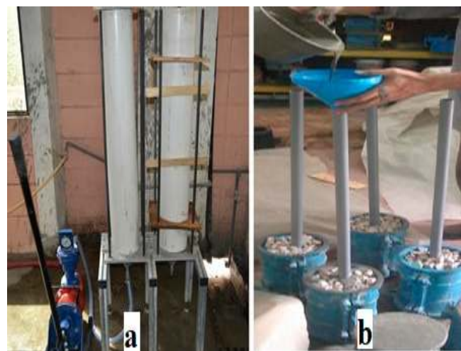
Figure 1. Grouting techniques of PAFRC: (a) Pumping; (b) Gravity.
