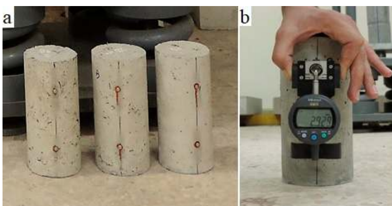
Figure 3. (a) PAFRC specimens used for drying shrinkage; (b) A digital comparator meter.
