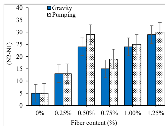
Figure 5. Variation of impact resistance values of PAFRC specimens vs. fiber content.
