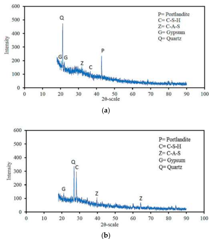
Figure 9. The X-Ray Diffraction (XRD) results of grout paste used in PAFRC specimens at (a) 28-day; (b) 90-day.
