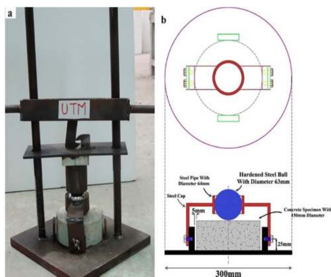
Figure 2. (a) The drop weight impact resistance device; (b) The test setup.
