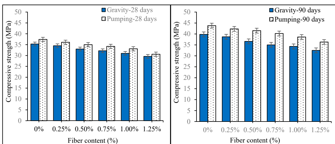
Figure 4. The variation in the compressive strength of PAFRC specimens.
