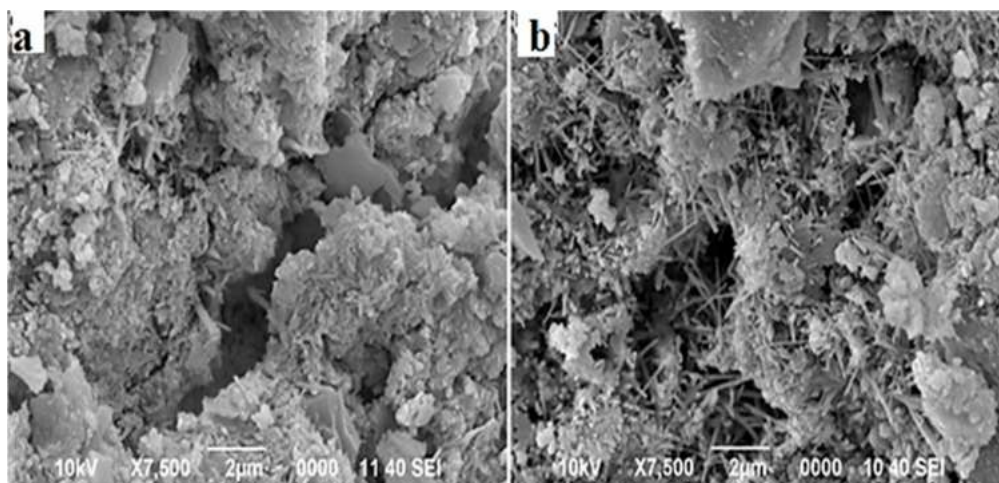
Figure 8. SEM images of (a) 28-day and (b) 90-day grout pastes used in PAC.
