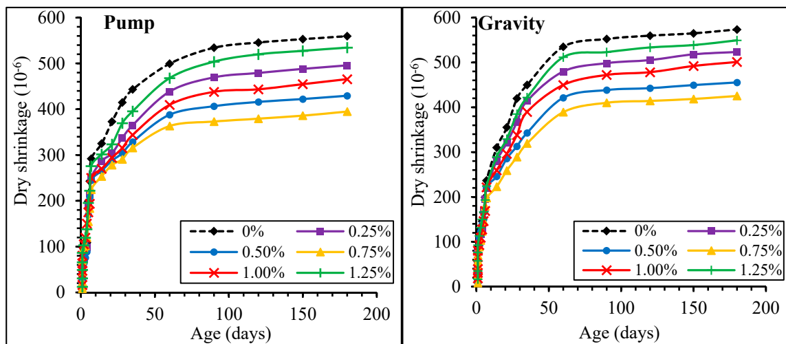
Figure 7. Drying shrinkage of PAFRC specimens.
