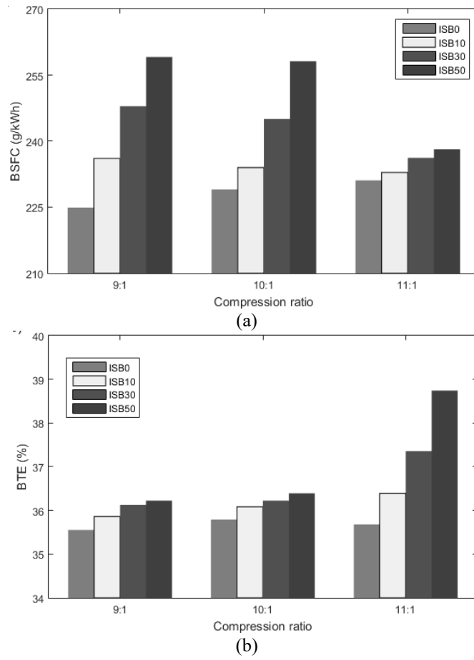
Figure 1. Variations of (a) BSFC and (b) BTE on CR, adapted from [88].
