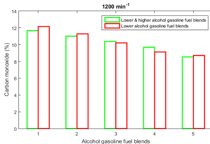
Figure 5. CO emission of various alcohol blends, adapted from [91].
