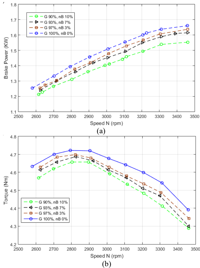
Figure 2. Power and torque against engine speed, adapted from [86].
