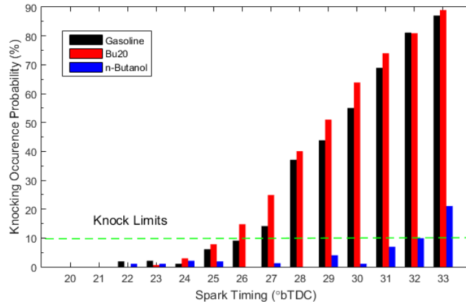
Figure 4. Knocking occurrence probability of butanol/gasoline blends, adapted from [83].
