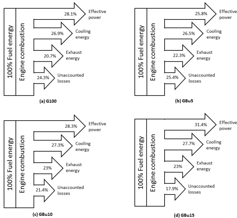
Figure 3. Sankey diagram of energy distribution for gasoline engine fuelled with (a) pure gasoline, (b) 5% butanol, (c) 10% butanol and (d) 15% butanol, adapted from [92].
