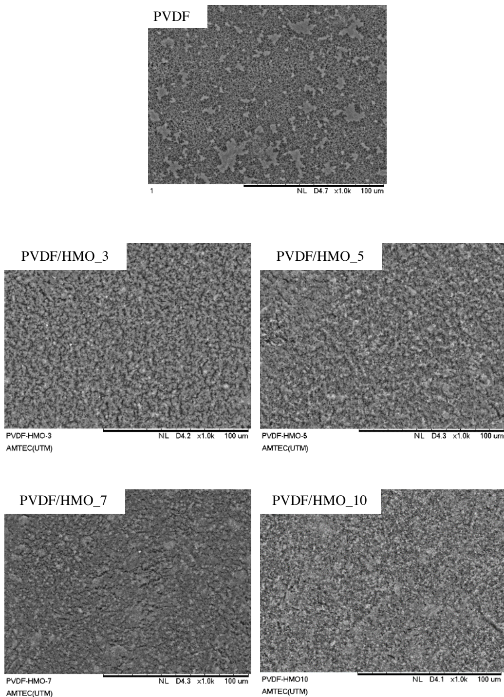
Figure 1: SEM images of pristine PVDF membrane and PVDF/HMO MMM top surface view
