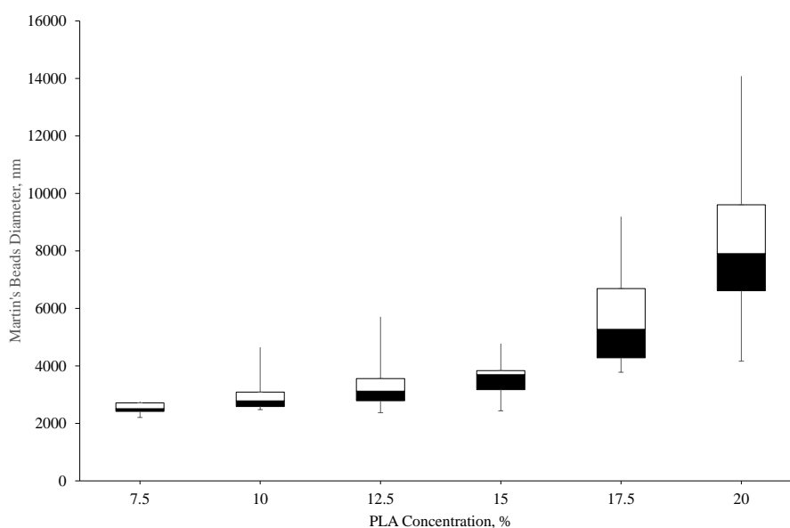
Figure 3: Box and whisker plot of beads diameter for 7.5–20 % w/v PLA concentrations.
