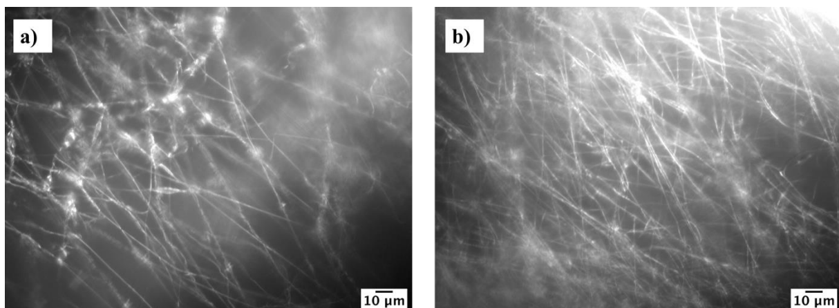
Figure 2: Electrospun fibres of PLA/DMF a) PLA concentration of 12.5 % w/v and b) PLA concentration of 15 % w/v.
