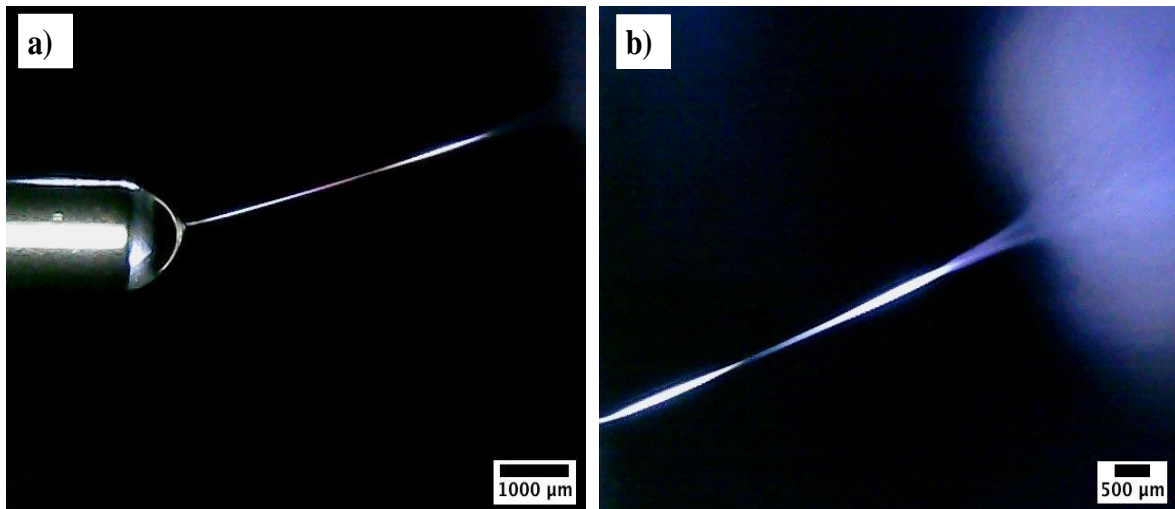
Figure 1: Electrospinning jet of 12.5 % w/v PLA concentration in PLA/DMF solution, a) Taylor cone at the tip of the needle and b) electrospinning plume.
