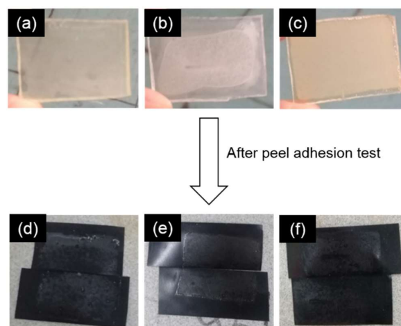
Figure 4. Images of TiO_2 coated by drop-casting method on PC sheets before (a-c) and after (d-f) peel adhesion test.
