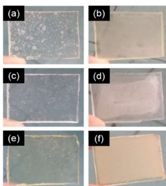
Figure 1. Thin films of TiO 2 coated on PC sheets; (a) TiO 2 suspension prepared by method 1 was spray-coated onto PC sheets, (b) TiO 2 suspension prepared by method 1 was drop-casted onto PC sheets, (c) TiO 2 suspension prepared by method 2 was sprayed-coated onto PC sheets, (d) TiO 2 suspension prepared by method 2 was drop-casted onto PC sheets, (e) TiO 2 suspension prepared by method 3 was sprayed-coated onto PC sheets and (f) TiO 2 suspension prepared by method 3 was drop-casted onto PC sheets.
