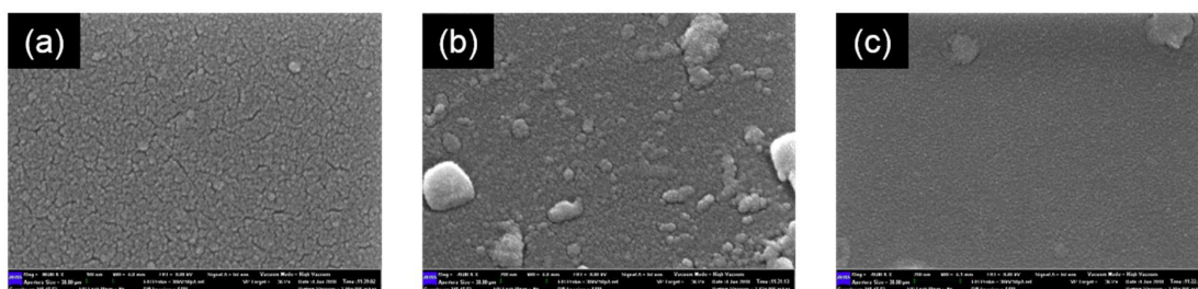
Figure 5. FESEM images PC sheets modified by APTMS followed by coating via drop-casting method with TiO 2 suspension prepared by (a) method 1 with magnification of 50000 times, (b) method 2 with magnification of 70000 times and (c) method 3 with magnification of 70000 times, all with accelerating voltage of 5.0 kV.
