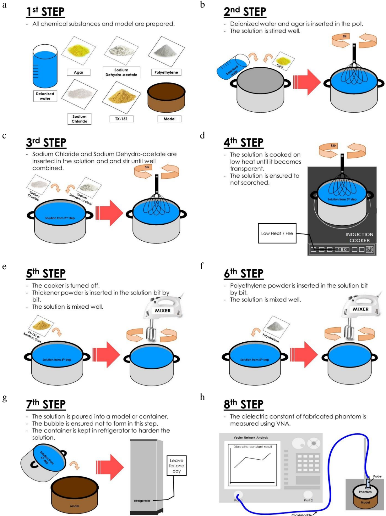
Fig. 1 - (a) First step; (b) second step; (c) third step; (d) fourth step; (e) fifth step; (f) sixth step; (g) seventh step; (h) eighth step
