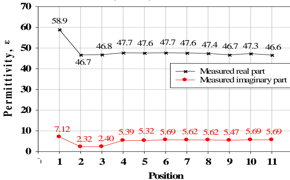
Fig. 4 - Measured value of real part, \epsilon' (re) and the imaginary part, \epsilon'' (im) of permittivity on the bottom surface of skin phantom
