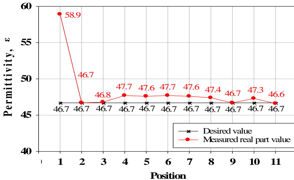
Fig. 5 - Comparison results of desired and measured permittivity, \epsilon_r for the bottom surface of skin phantom
