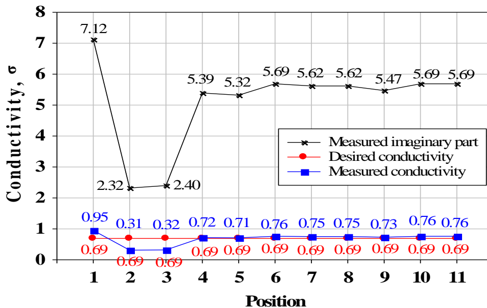
Fig. 6 - Comparison results of desired and measured conductivity, \sigma for the bottom surface of skin phantom
