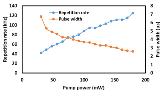
Figure 6. Pulse repetition rate and pulse width versus pump power
