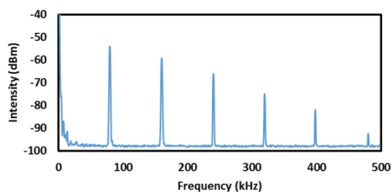
Figure 8. RFSA measurement of signal to noise ratio Graphene slurry based SA of 44 dB with 500 kHz span
