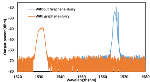
Figure 4. OSA trace with and without Graphene slurry based SA
