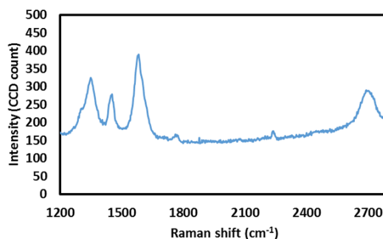
Figure 2. Raman spectroscopy of Graphene slurry
