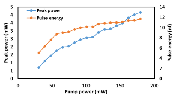
Figure 7. Peak power and pulse energy versus pump power
