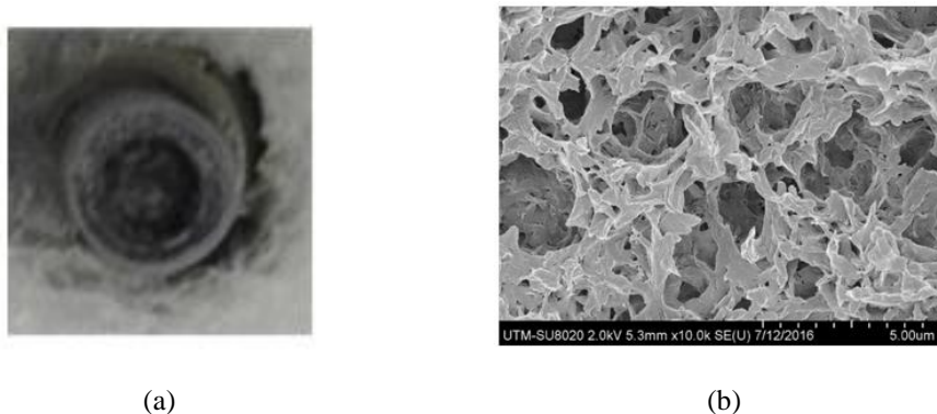
Figure 1. (a) Graphene slurry at the end of fiber ferrule, (b) FESEM image of Graphene slurry
