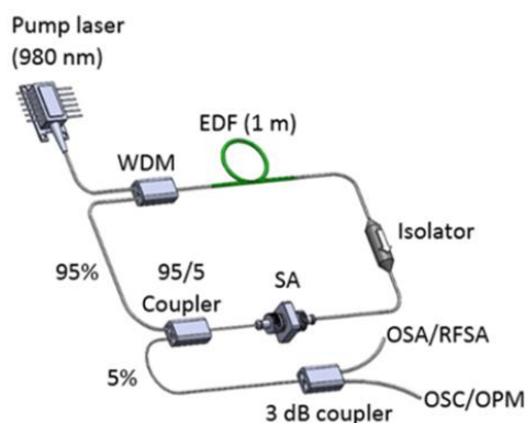
Figure 3. Integration of Graphene slurry based SA in fiber laser in ring cavity; OSA-optical spectrum analyzer, RFSA-Radio frequency spectrum analyzer, OSC-oscilloscope, OPM-optical power meter
