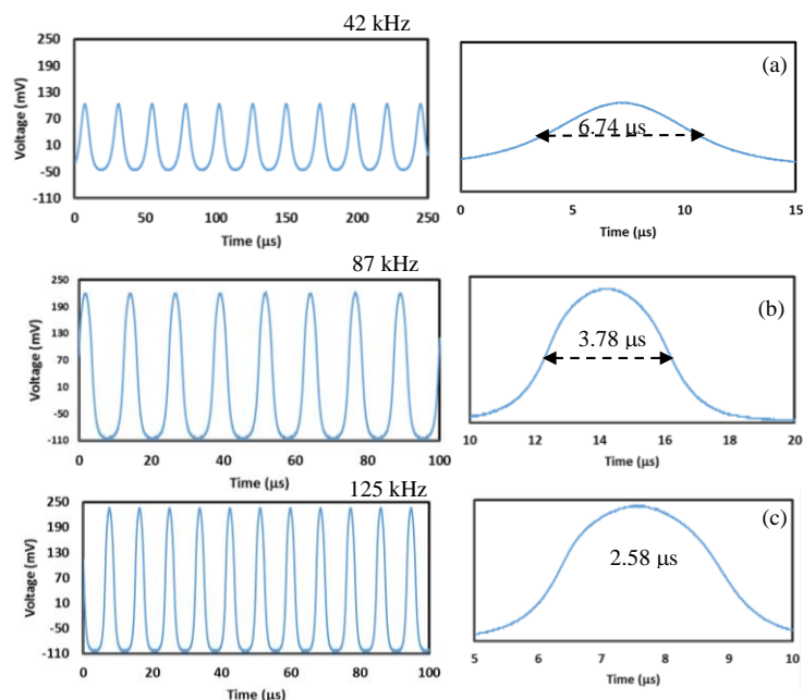
Figure 5. Pulse train and pulse width at input pump power, (a) 30.4 mW, (b) 100 mW, and (c) 179.4 mW
