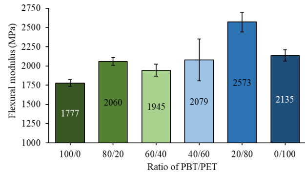
Figure 9 Flexural modulus of PBT, PET and PBT/PET blends
