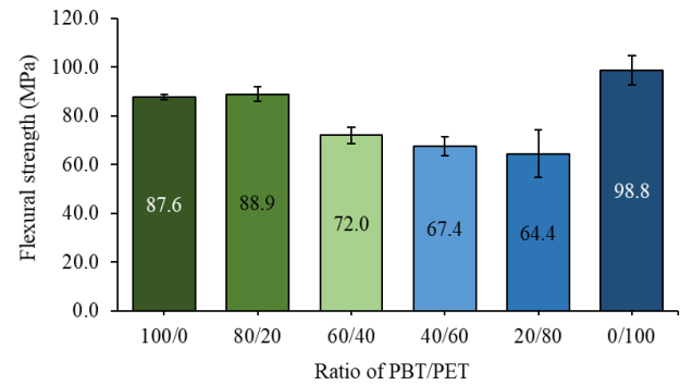
Figure 8 Flexural strength of PBT, PET and their blends
