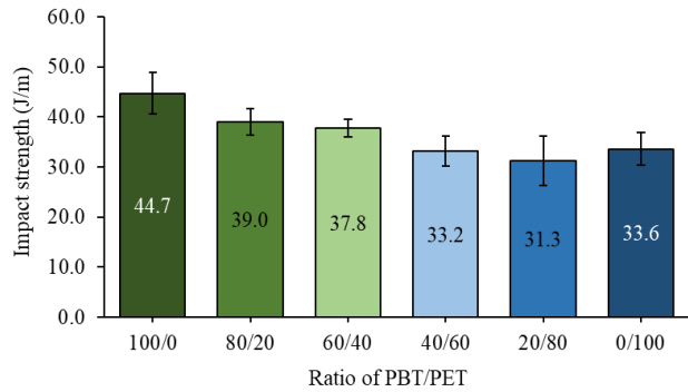
Figure 10 Impact strength of PBT, PET and PBT/PET blends
