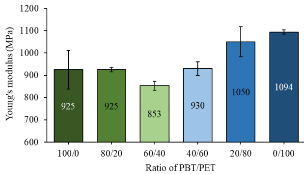
Figure 6 Young's modulus of PBT, PET and PBT/PET blends
