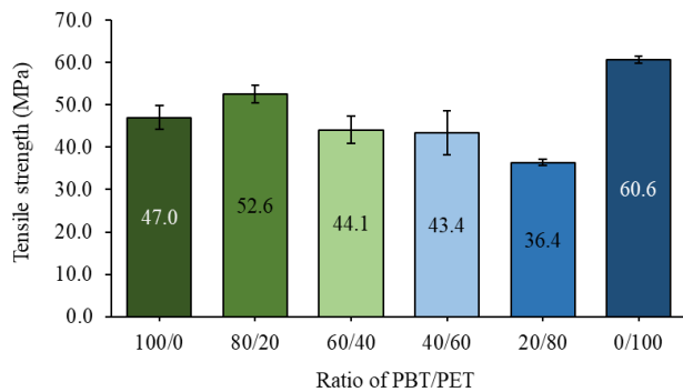
Figure 5 Tensile strength of PBT, PET, and PBT/PET blends
