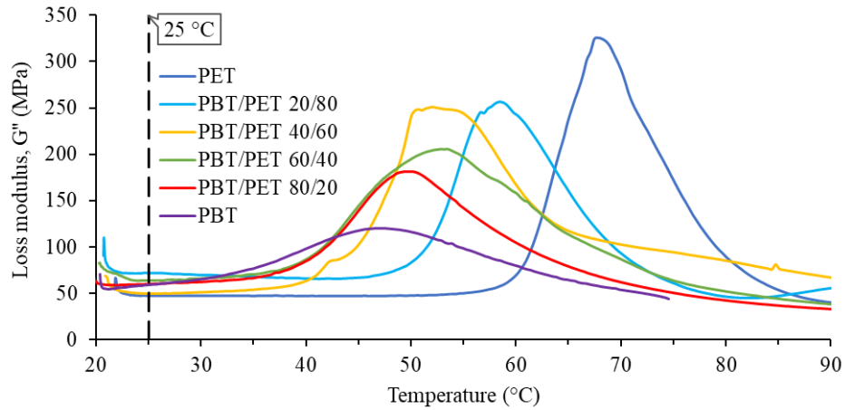
Figure 3 Loss modulus of PBT/PET blends
