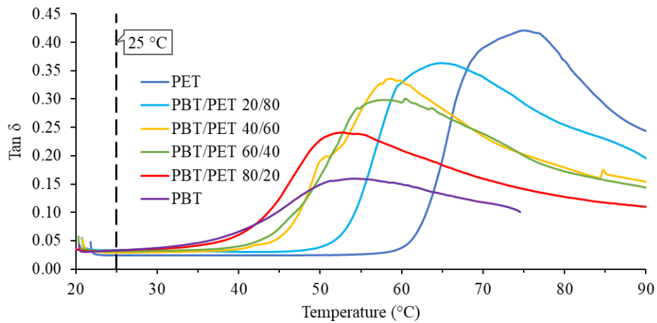
Figure 4 Tan delta of PBT/PET blends
