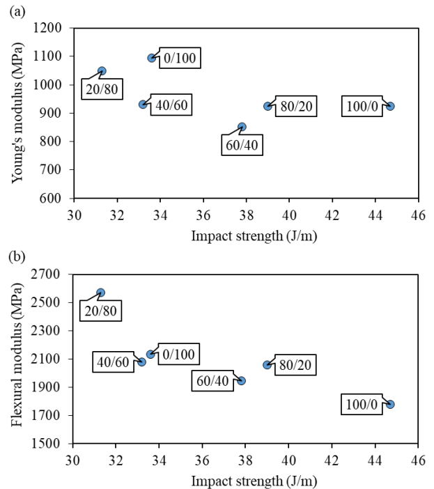
Figure 11 Properties of PBT, PET and PBT/PET blends in terms of stiffness and toughness (a) Young's modulus and impact strength (b) flexural modulus and impact strength
