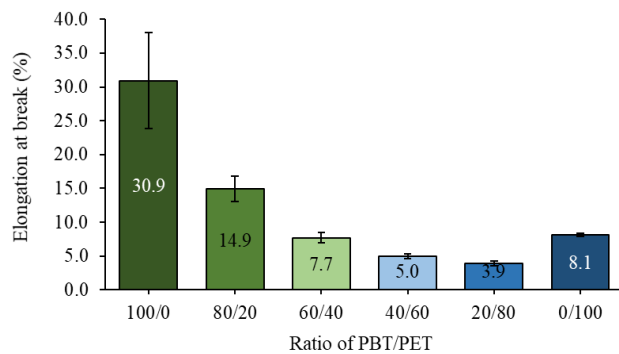
Figure 7 Elongation at break of PBT, PET and their blends
