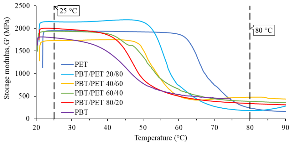
Figure 2 Storage modulus of PBT/PET blends
