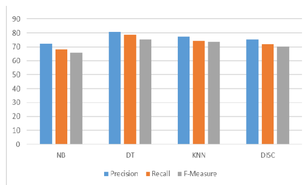
Fig. 1. Precision, Recall and F-Measure values for CFS
