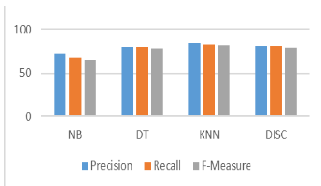
Fig. 6. Precision, Recall and F-Measure values for DE
