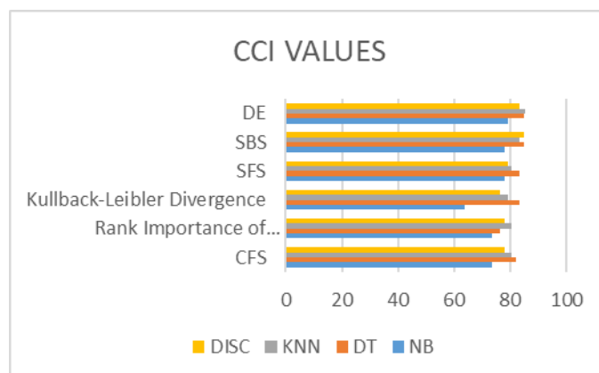
Fig. 7. CCI Values for FS Algorithms
