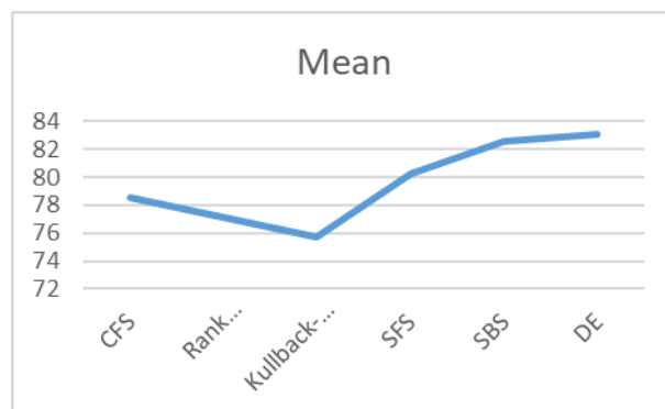
Fig. 8. Mean Values for FS Algorithms
