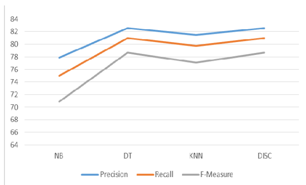
Fig. 5. Precision, Recall and F-Measure values for SBS
