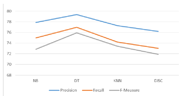
Fig. 4. Precision, Recall and F-Measure values for SFS
