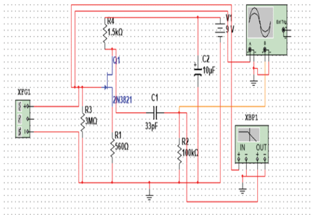
Fig. 1: Schematic diagram of PZT preamplifier
