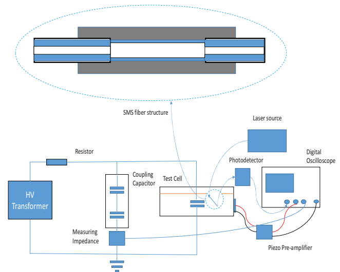
Fig. 3: PD measurement test set up
