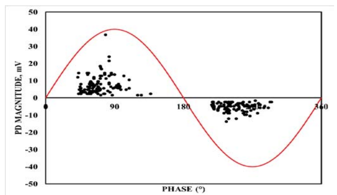
Fig 6: Detected PD using pre-amplified Piezoelectric Diaphragm
