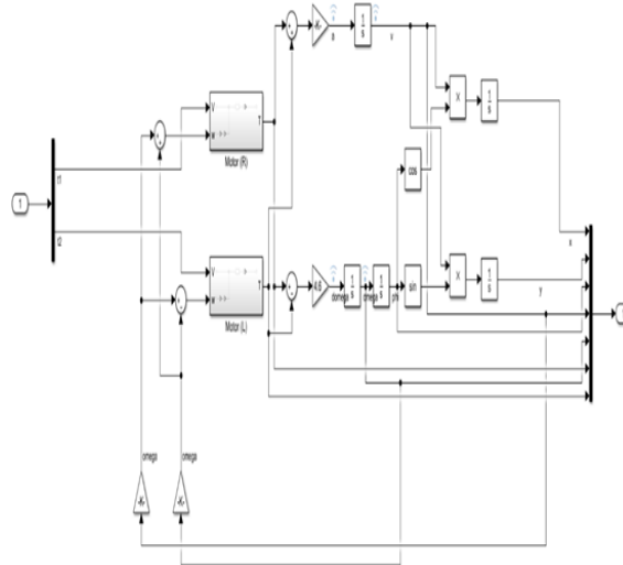
Figure 6. Simulink Model of the subsystem.
