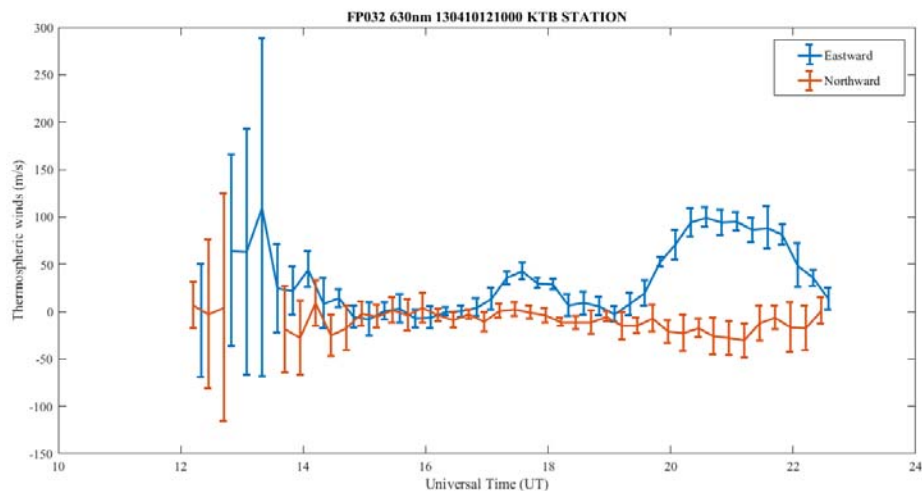
Figure 3. Temporal variation of thermospheric neutral winds observed by FPI at KTB station.
