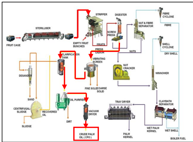
Figure 3: Palm Oil Mill Flow Process Diagram
