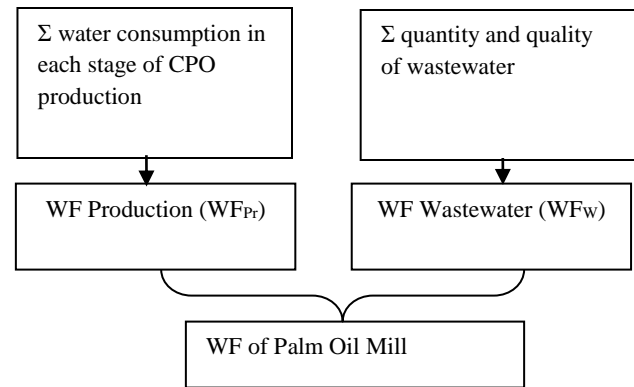
Figure 2: The Calculation Method of WF at Palm Oil Mill
