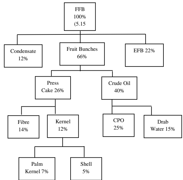
Figure 5: Material balance for 1 t CPO production
