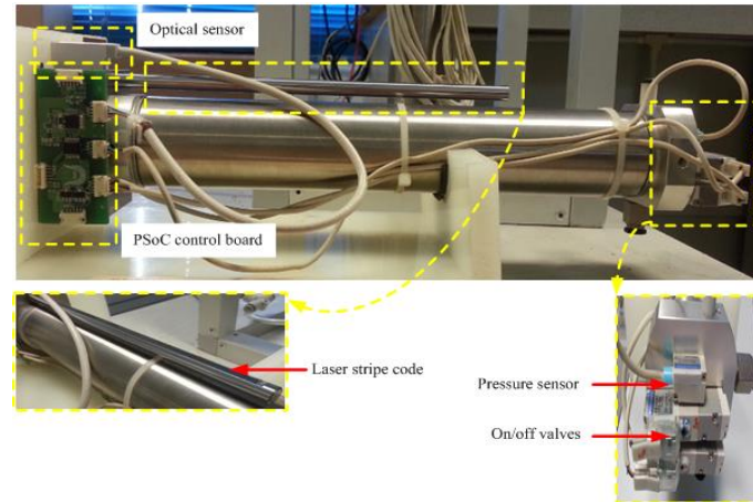
Figure 1. The pneumatic actuator system
