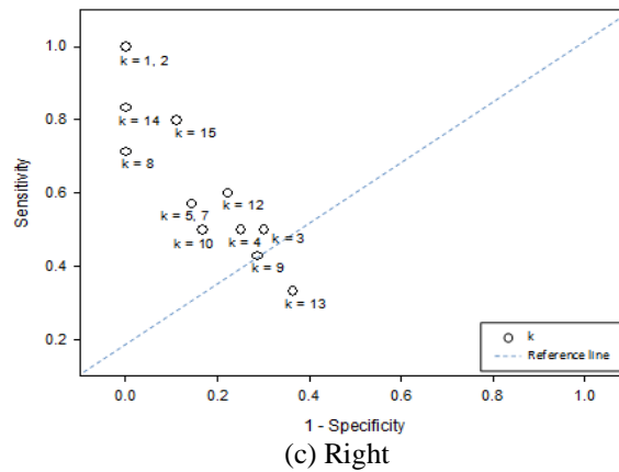
Figure 6. ROC Plot of Classifier 1
