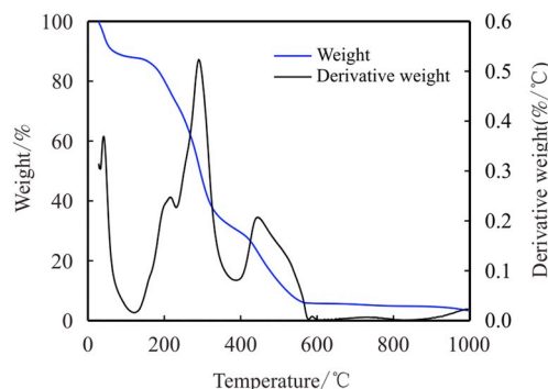
Fig. 3. TGA and DTGA curves of untreated DR.
