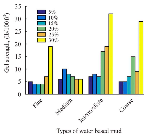
Fig. 13. Gel strength (10 s) for water-based mud with treated DR.
