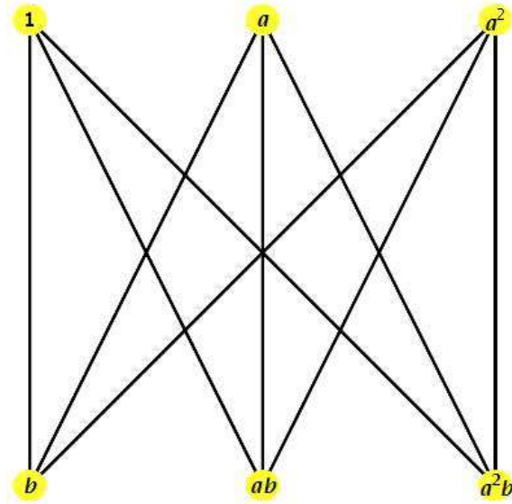
Figure 1: Cay(D_6, \{b, ab, a^2b\}) = K_{3,3}
