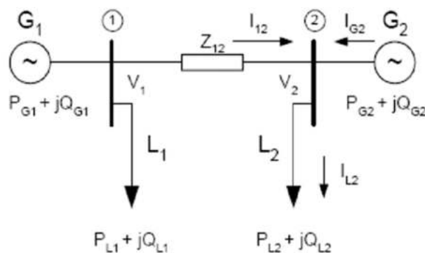
Figure 3. Bus test via distributed generation (DG) integration into network [41].
