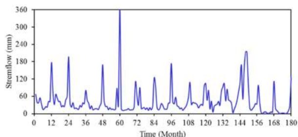
FIGURE 2. Streamflow time series of Pahang River at a station 3527410.
