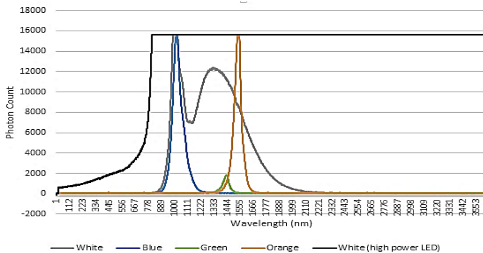
Figure 2. Spectrometer output
