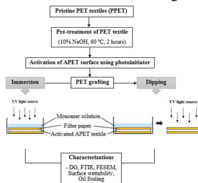
Fig. 1. Flow chart of the experimental design outline which consists of pre-treatment step of PPET, surface activation of APET using photoinitiator, grafting of APET via immersion and dipping methods and the characterization of post-cured APET textiles.
