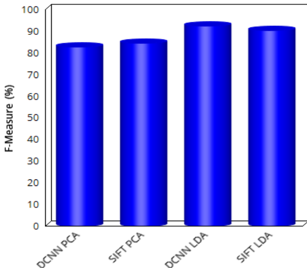
Fig. 4 F-Measure assessment
