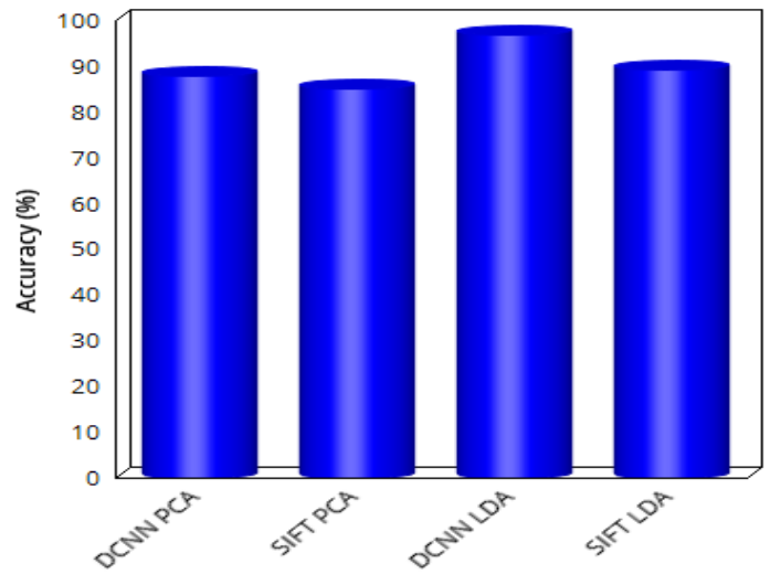
Fig. 2 Accuracy assessment
