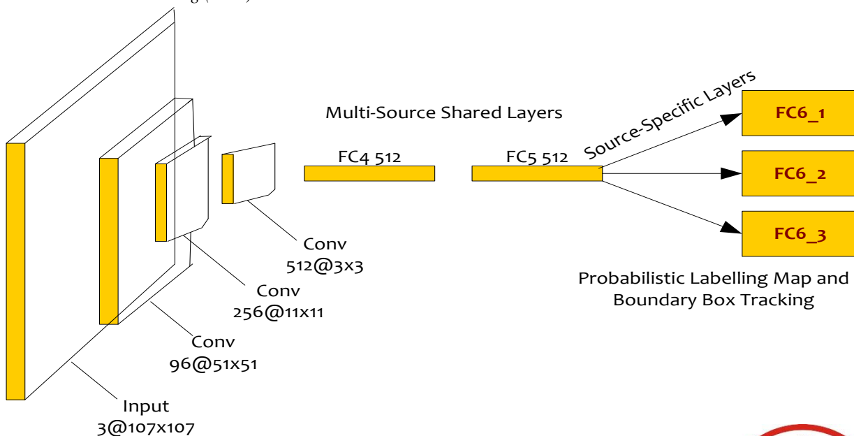
Fig. 1 The architecture of DCNN based vehicle detection and tracking
