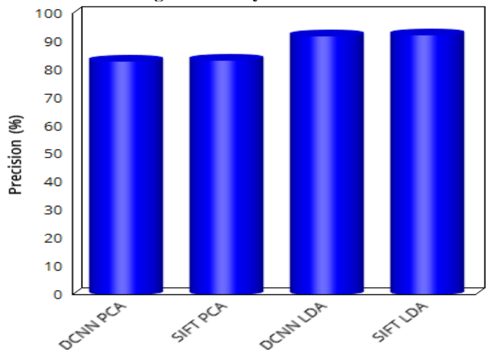
Fig. 3 Precision assessment
