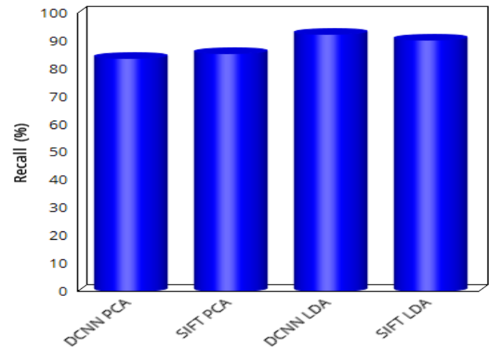
Fig. 4 Recall assessment
