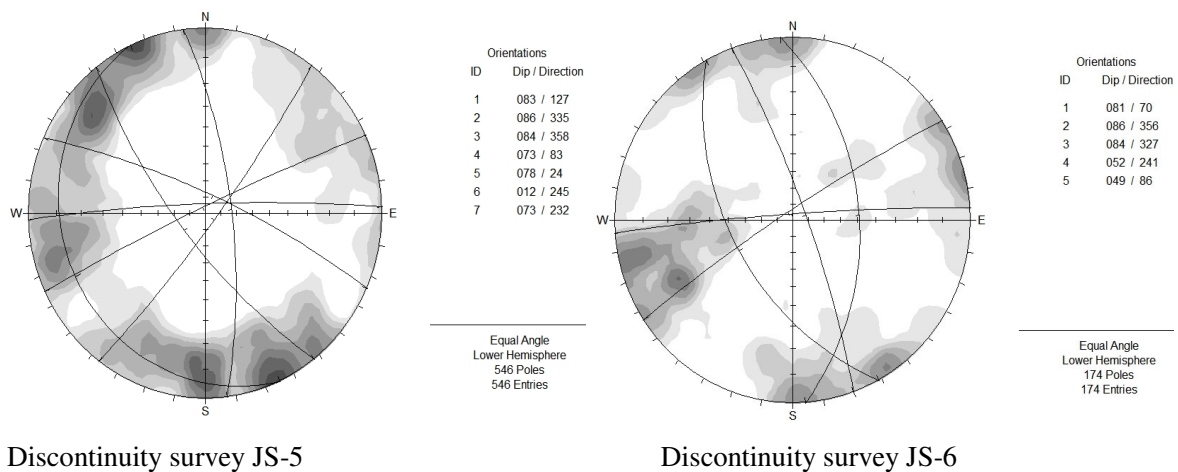
Figure 2. Stereographic projection.
