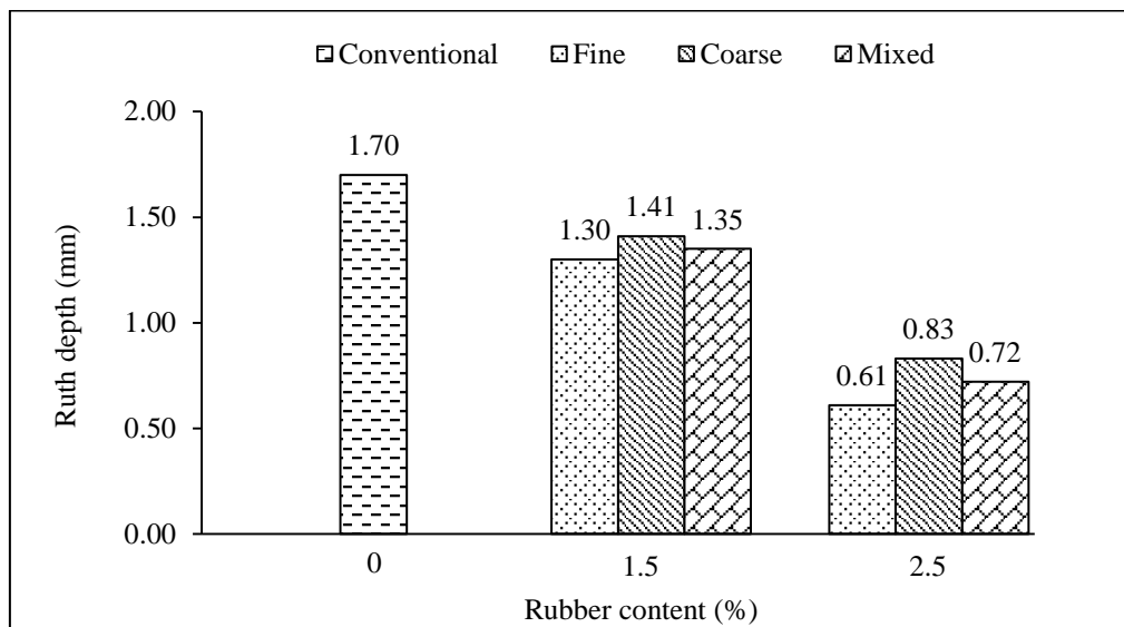
Figure 7. Dynamic creep test.
