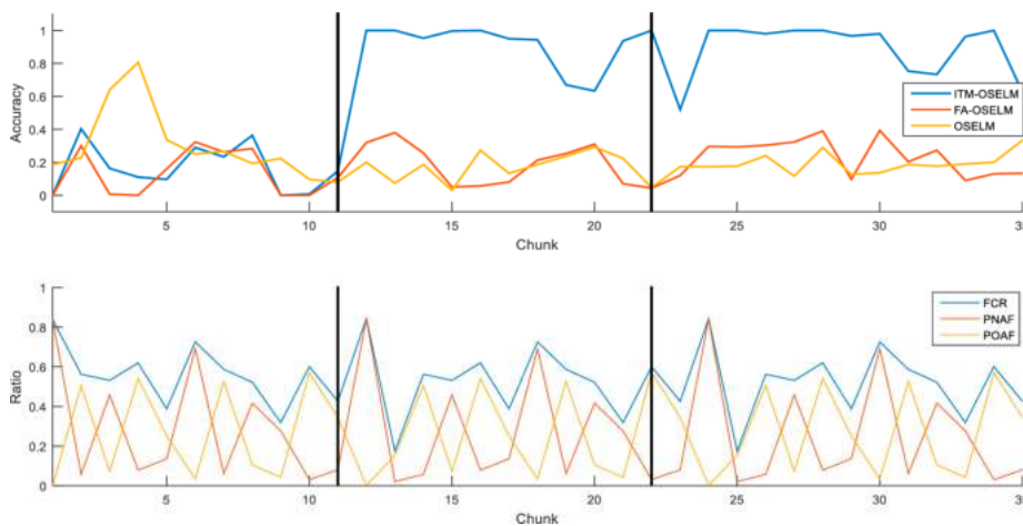
Figure 7. Accuracy change with respect to data chunks for three cycles using the UJIndoorLoc dataset.
