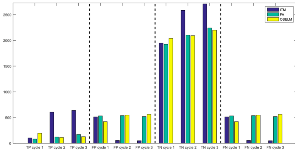
Figure 11. Classification measures with respect to cycles for the three models with the UJIndoorLoc dataset.
